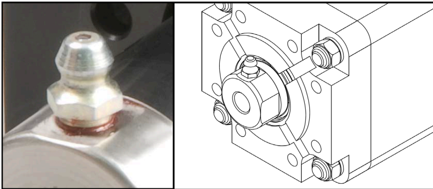
Figure 7.1: A standard grease zerk allows periodic relubrication for ServoWeld actuators. This can be done without removing the actuator from its installation.
